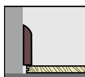
FINSkirting 80 x 16 x 2700mm
